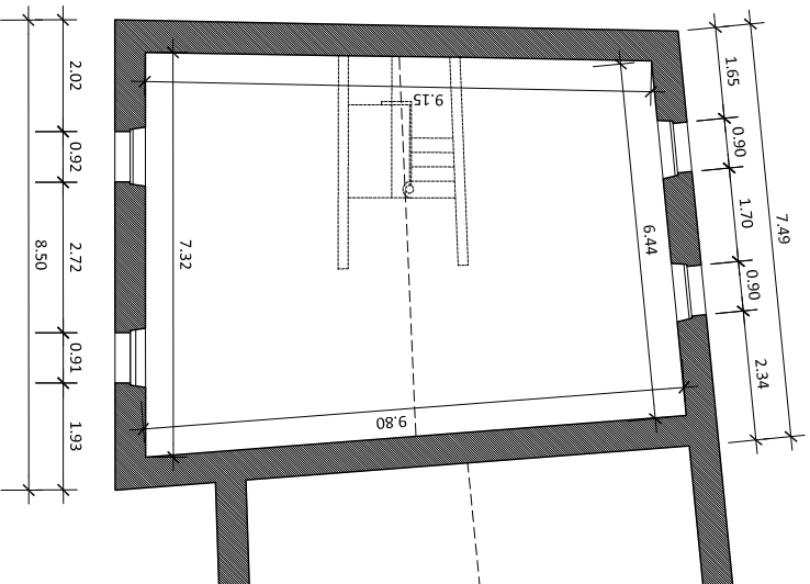
PLAN NIV. R+1 / 53.66 NGF
